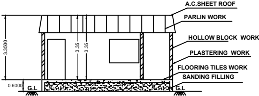
SECTION "AB"
