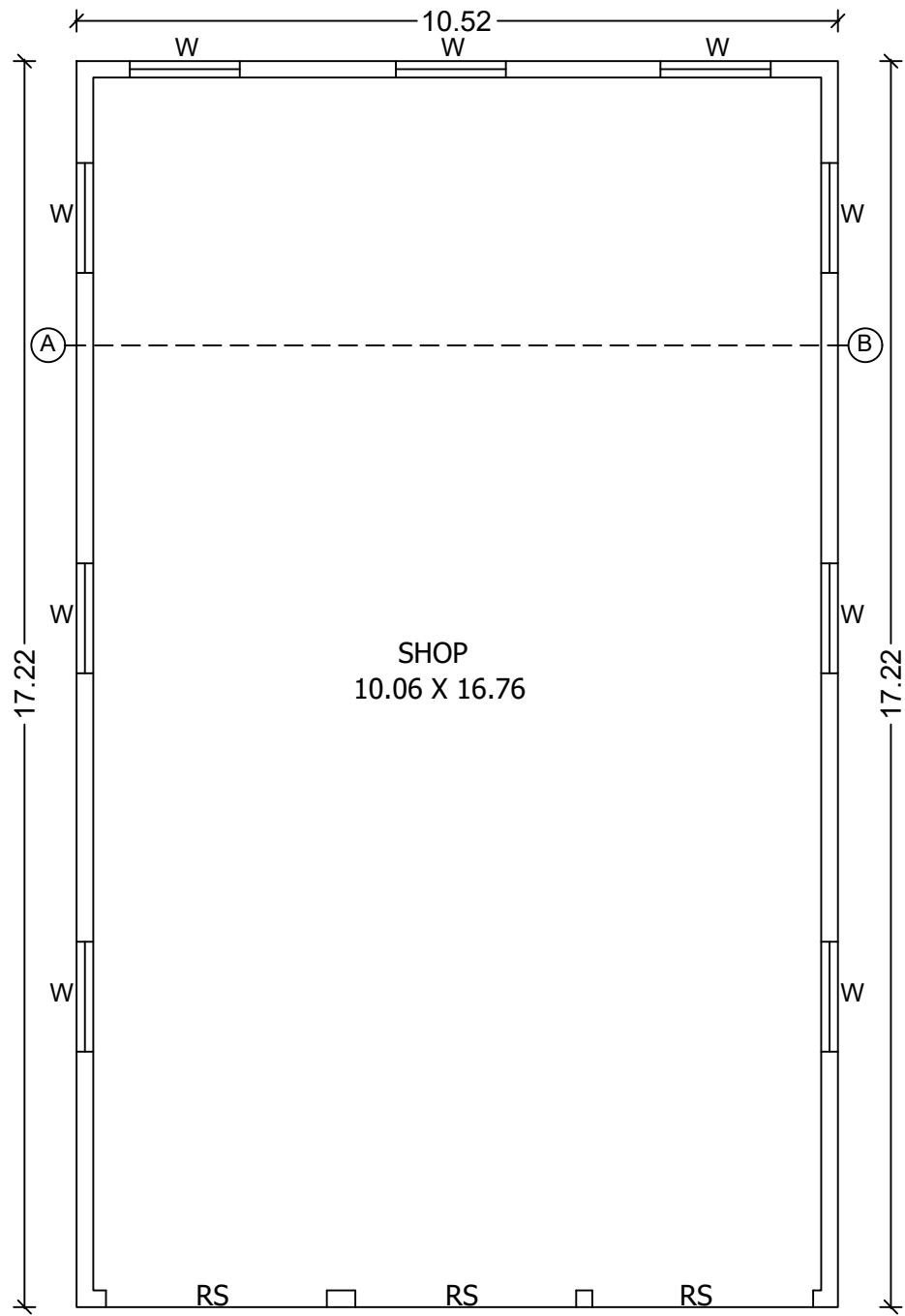
GROUND FLOOR PLAN EAST FACEING
