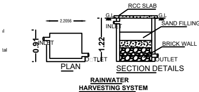
RAINWATER HARVESTING SYSTEM
