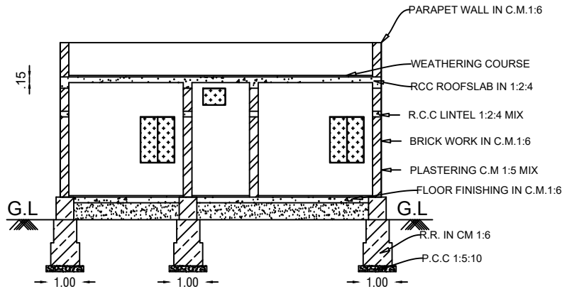
SECTION ON-"AB"
