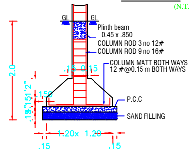
FOUNDATION DETAIL
