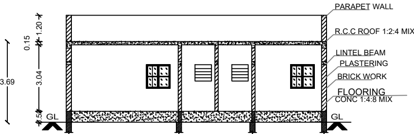
SECTION: A-B
