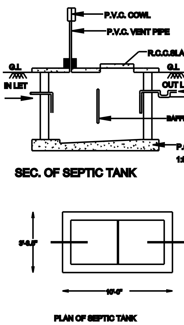
PLAN OF SEPTIC TANK
