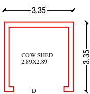
GROUND FLOOR
