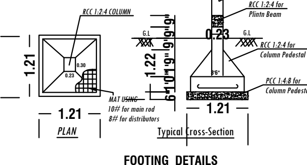
FOOTING DETAILS
