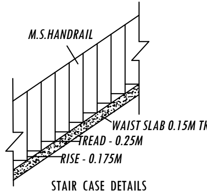
STAIR CASE DETAILS
