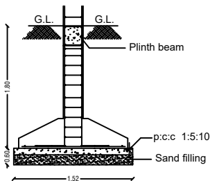
FOUNDATION DETAILS
