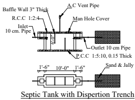
Septic Tank with Dispersion Trench
