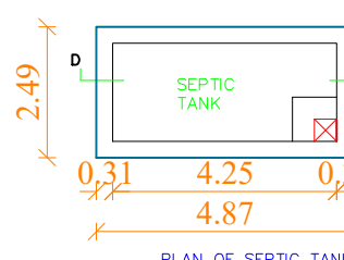
SEPTIC TANK
