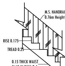
STAIRCASE DETAILS SCALE-1:20
