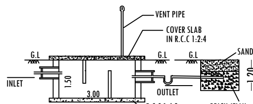
SECTION-AB
