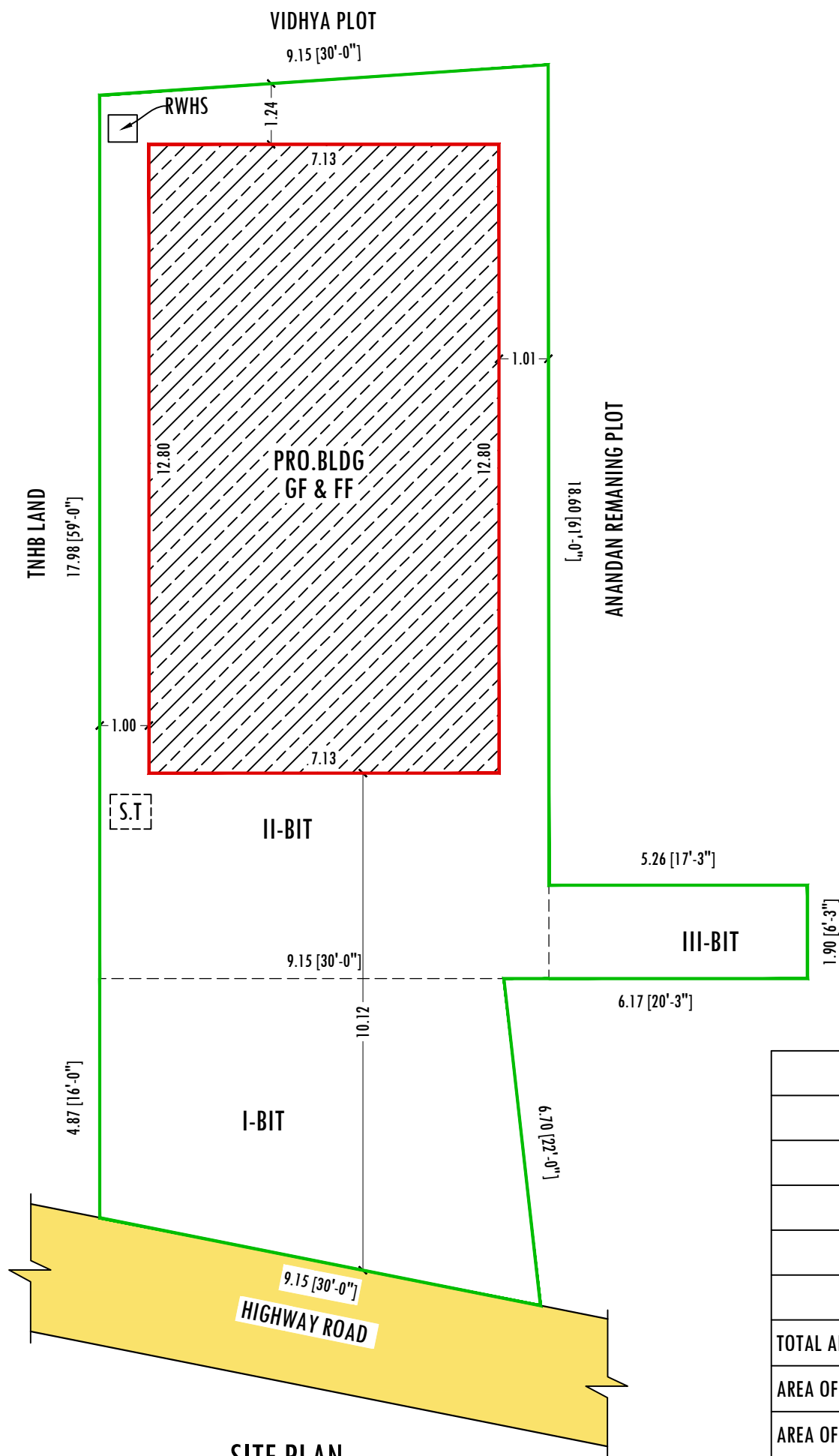
SITE PLAN
