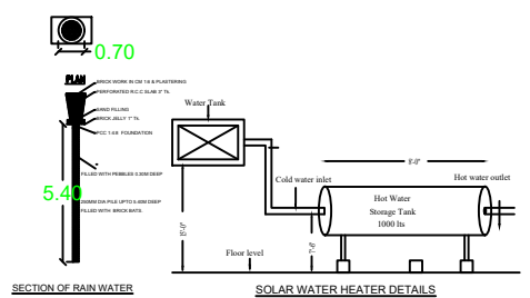
SOLAR WATER HEATER DETAILS
