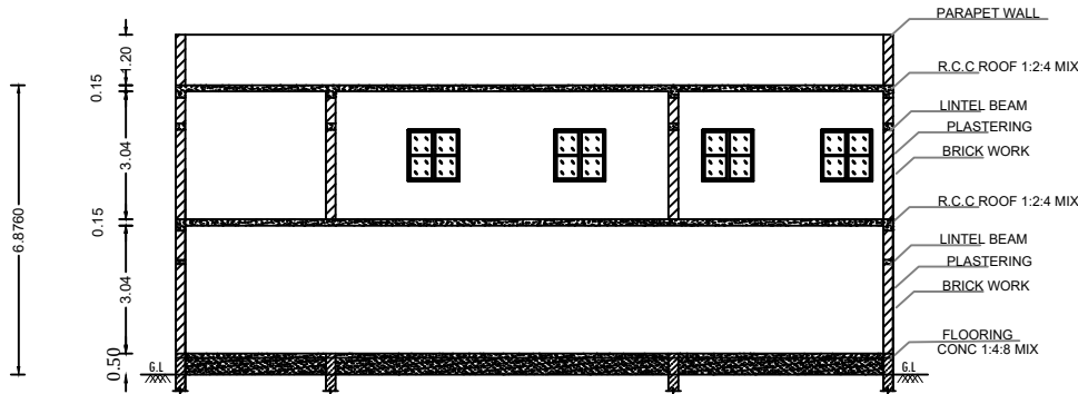
SECTION : "A-B"
