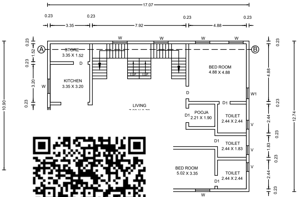
FLOOR PLAN
