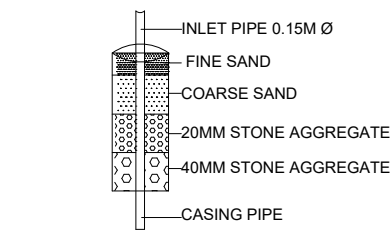
DETAILS OF RAIN WATER HARVESTING STRUCTURES
