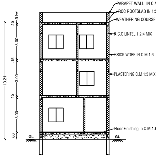
SECTION ON-'AB''
