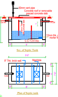
Plan of Septic tank
