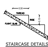
STAIRCASE DETAILS
