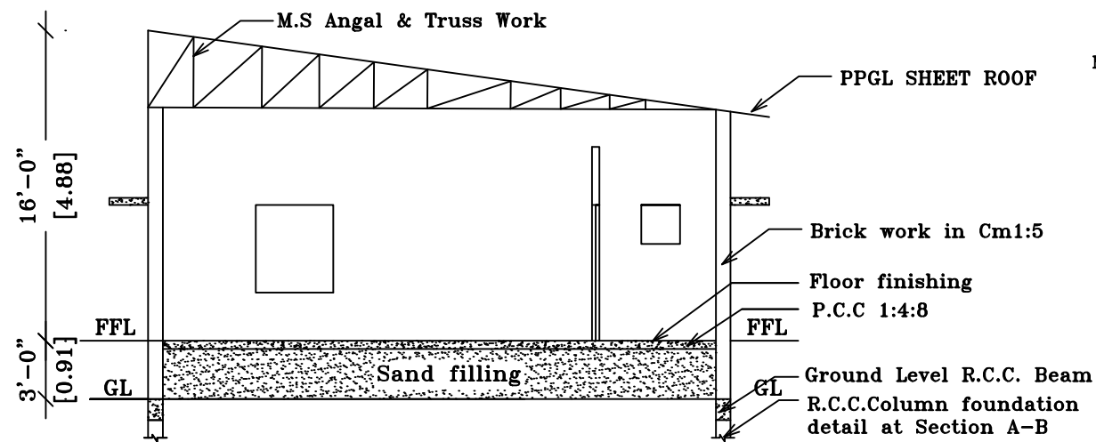
SECTION ON 'SA'
