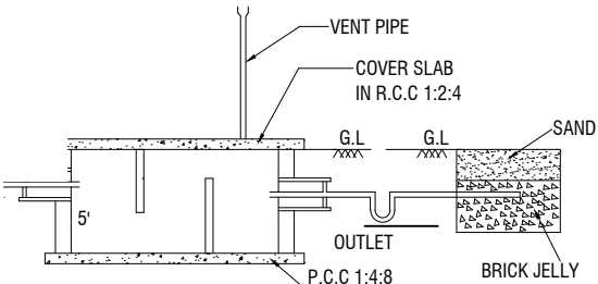
SECTION-AB
