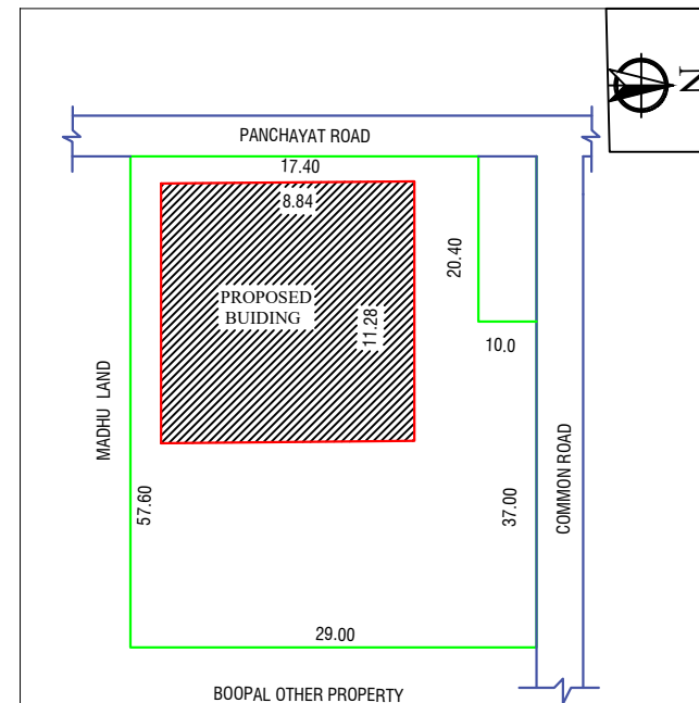
SIT PLAN
