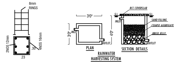
COLUMN DETAILS
