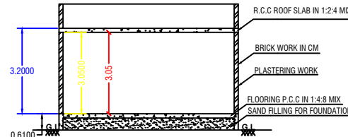
SECTION ON-AB
