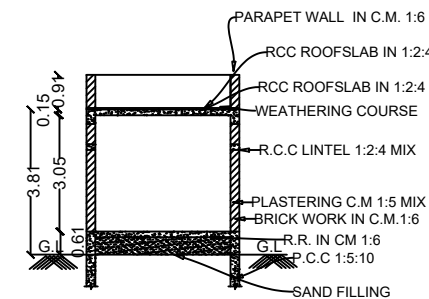
Section On-'AB'
