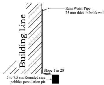
RAINWATER HARVESTING
