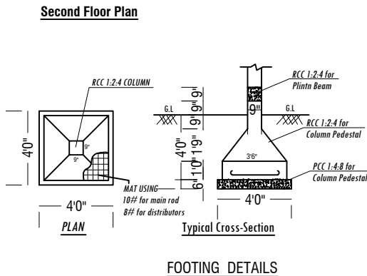
FOOTING DETAILS
