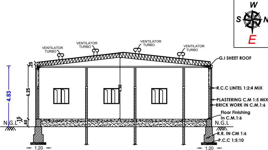
Section on-"AB"
