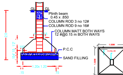
FOUNDATION DETAIL
