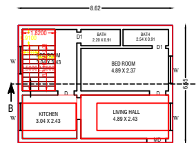
Proposed Ground Floor
