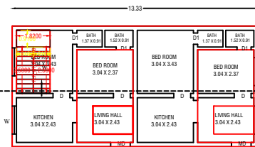
Proposed First Floor Plan
