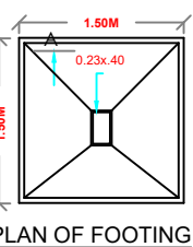
PLAN OF FOOTING
