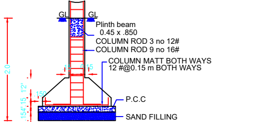
FOUNDATION DETAIL
