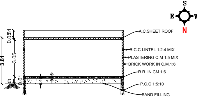
Section On-"AB"
