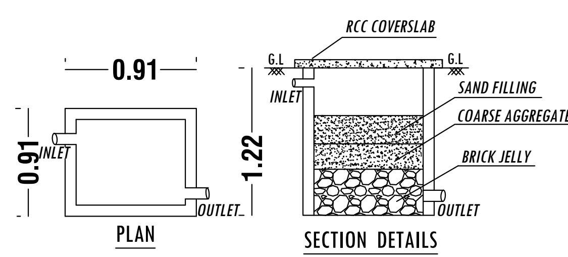
RAINWATER HARVESTING SYSTEM
