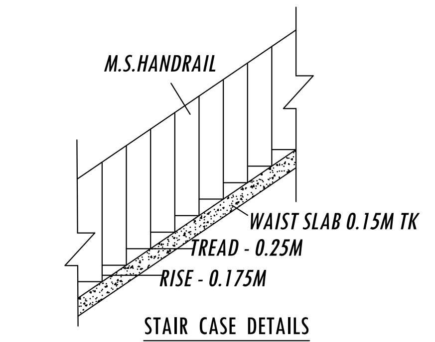
STAIR CASE DETAILS
