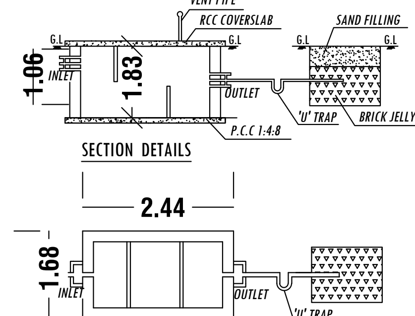
SECTION DETAILS
