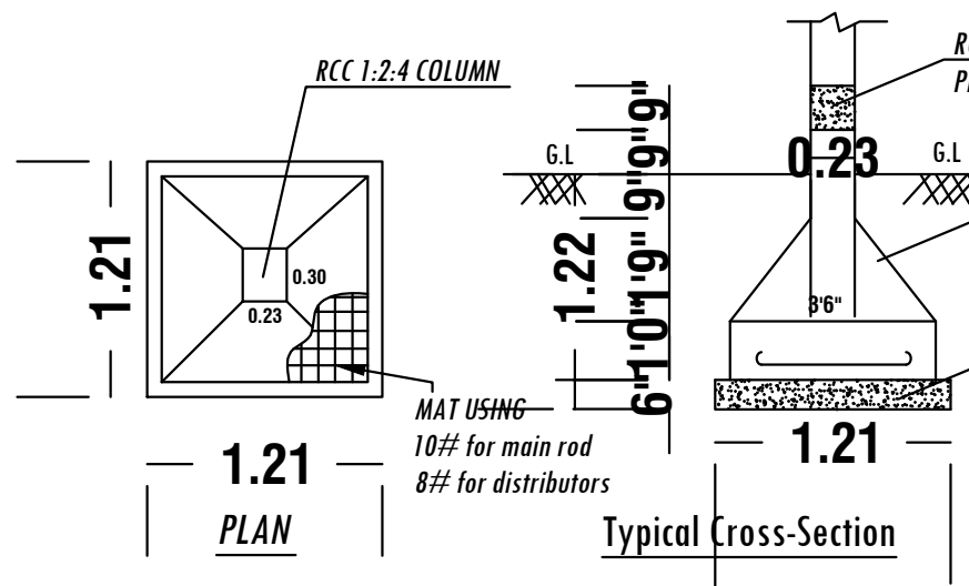
FOOTING DETAILS
