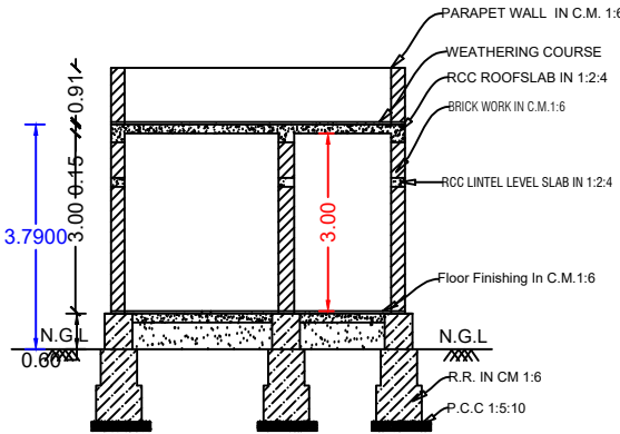
SECTION ON-"AB"
