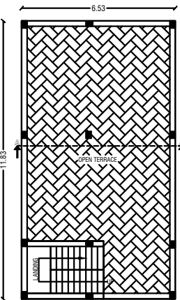
OPEN TERRACE FLOOR PLAN
