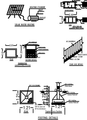
FOOTING DETAILS
