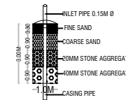
DETAILS OF RAIN WATER HARVESTING STRUCTURES
