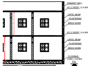
SECTION : "A-B"
