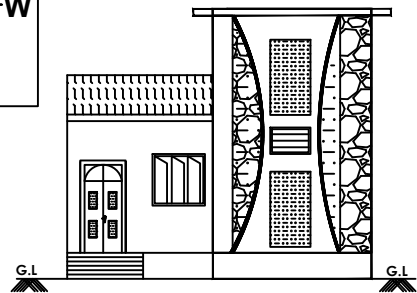
ELEVATION PLAN
