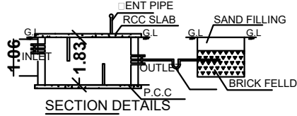
SECTION DETAILS
