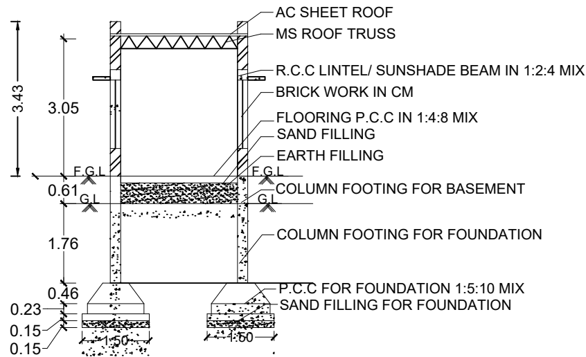
SECTION ON-AA
