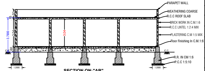
SECTION ON-"AB"
