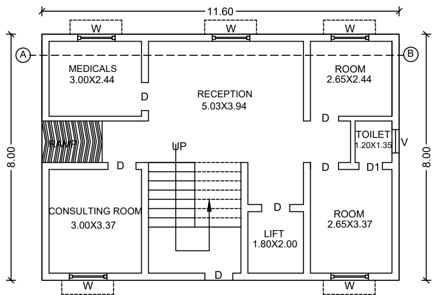
GROUND FLOOR PLAN EXISTING APPROVED
