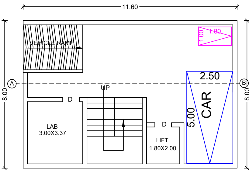
SEMI BASEMENT FLOOR PLAN EXISTING APPROVED
