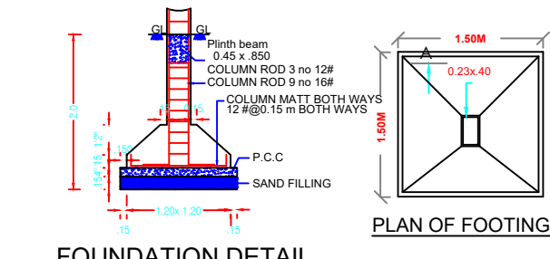
FOUNDATION DETAIL
