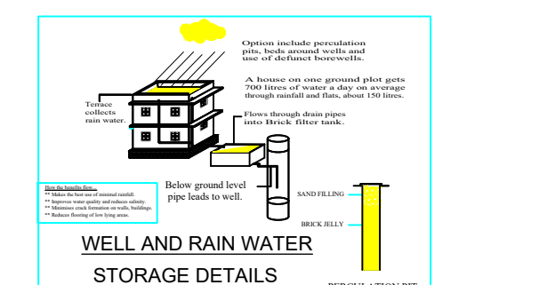
WELL AND RAIN WATER STORAGE DETAILS
