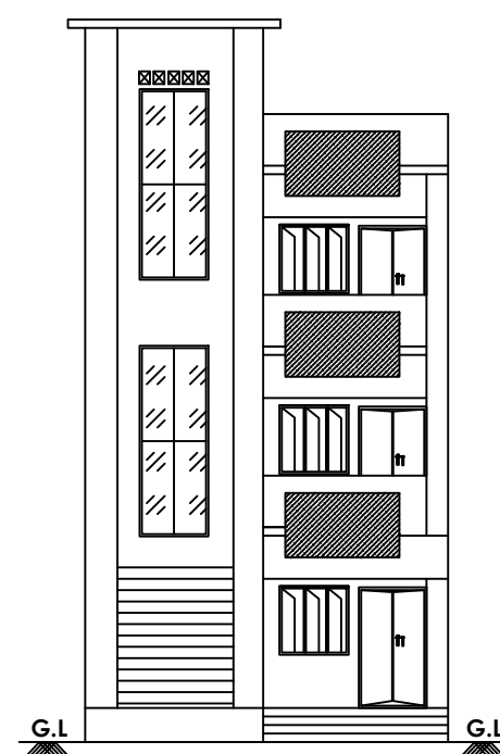
ELEVATION PLAN
