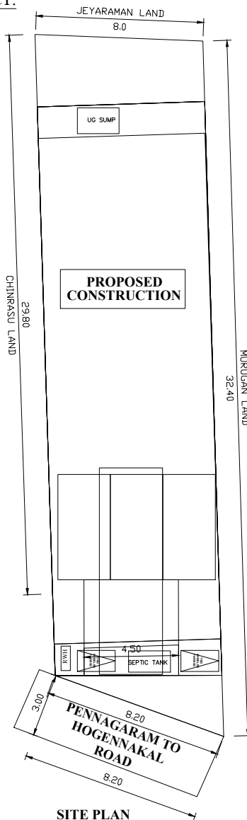
SITE PLAN
