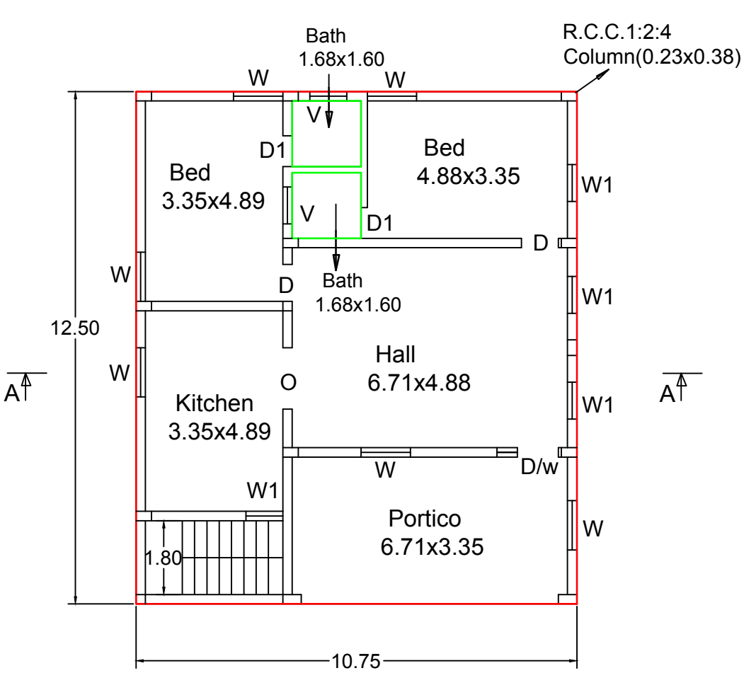
PLAN - Ground Floor
