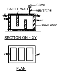
SEPTICTANK DETAILS NOT TO SCALE
