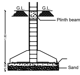
FOUNDATION DETAILS
