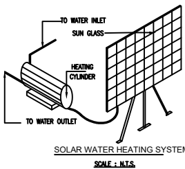
SOLAR WATER HEATING SYSTEM SCALE : MTS.
