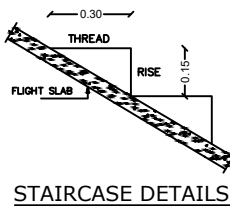
STAIRCASE DETAILS (NOT TO SCALE)
