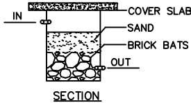
RAINWATER HARVEST NOT TO SCALE
