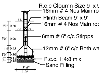
COLUMN DETIAL
