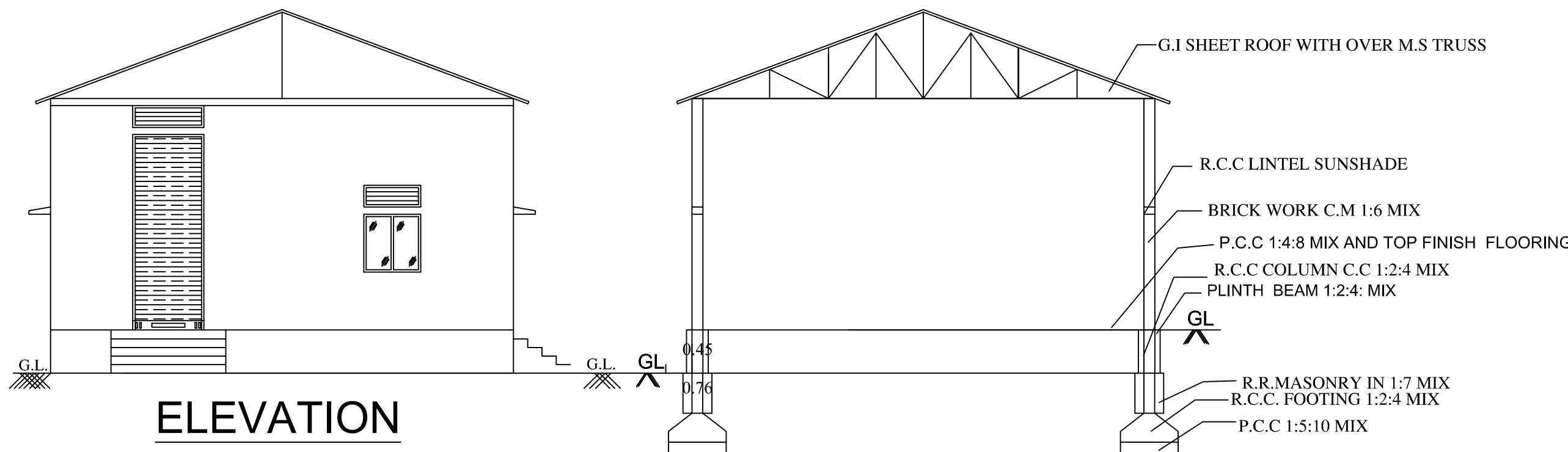
CROSS SECTION"AB"
