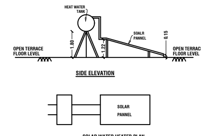
SOLAR WATER HEATER PLAN
