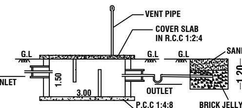
SECTION-AB
