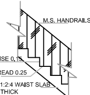
STAIRCASE DETAILS SCALE- 1:20
