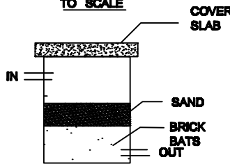
RAIN WATER DETAIL NOT TO SCALE
