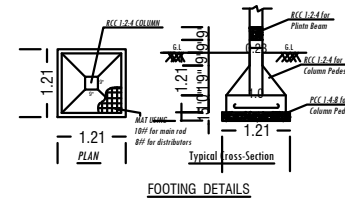
FOOTING DETAILS
