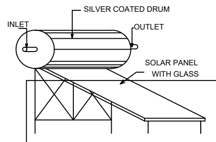
SOLAR SYSTEM
