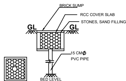
RAIN WATER HARVESTING TANK NOT TO SCALE
