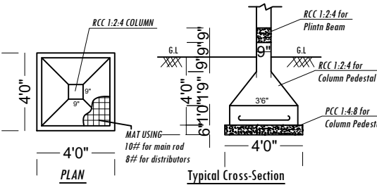
FOOTING DETAILS
