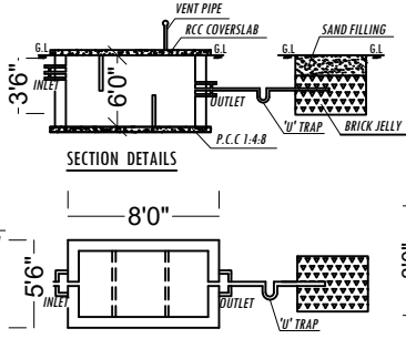
SEPTIC TANK AND DISPERSION TRENCH DETAILS
