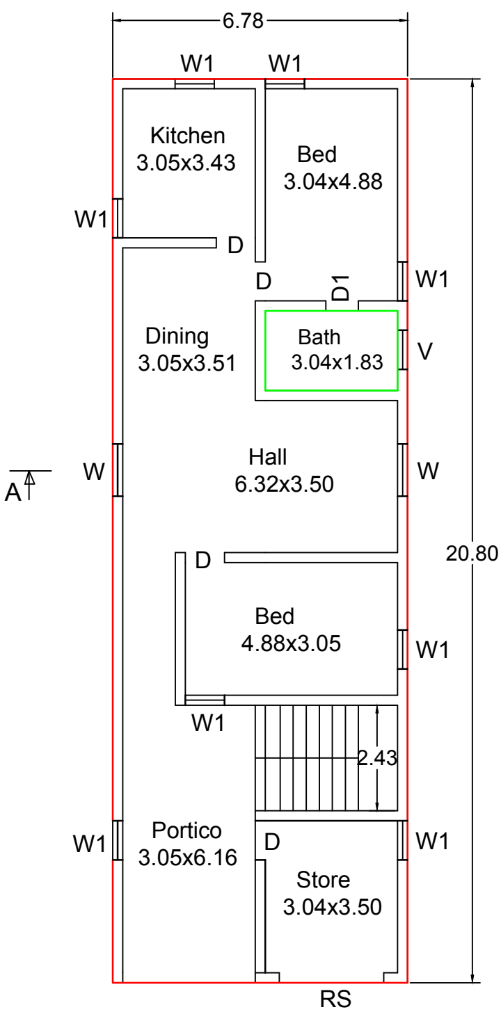
PLAN - Ground Floor
